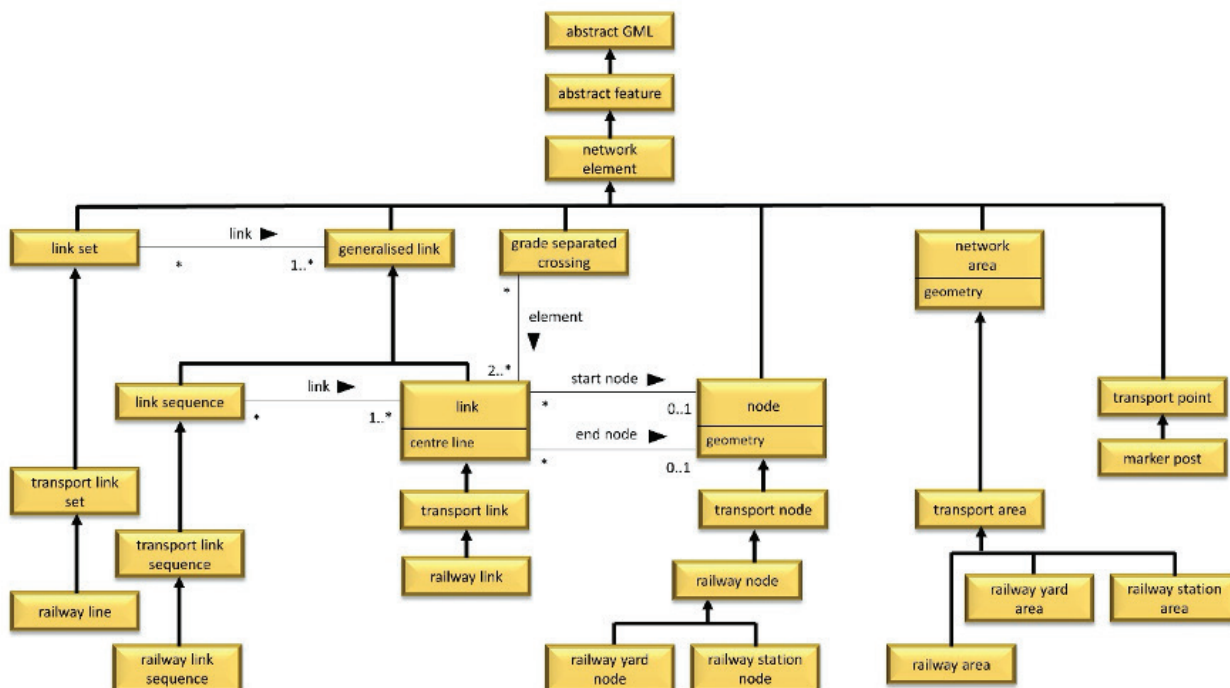
Figure 17 - Railway transport network
