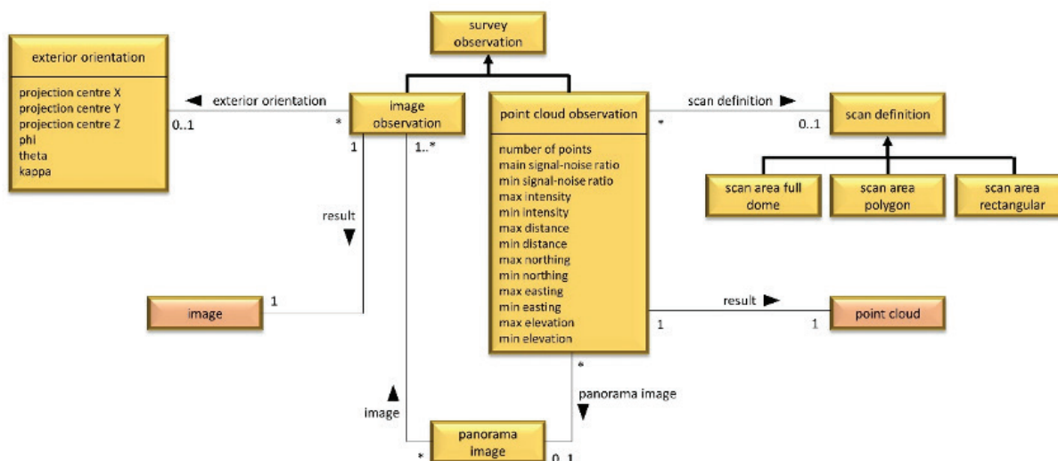
Figure 15 - LandInfra model for point cloud
