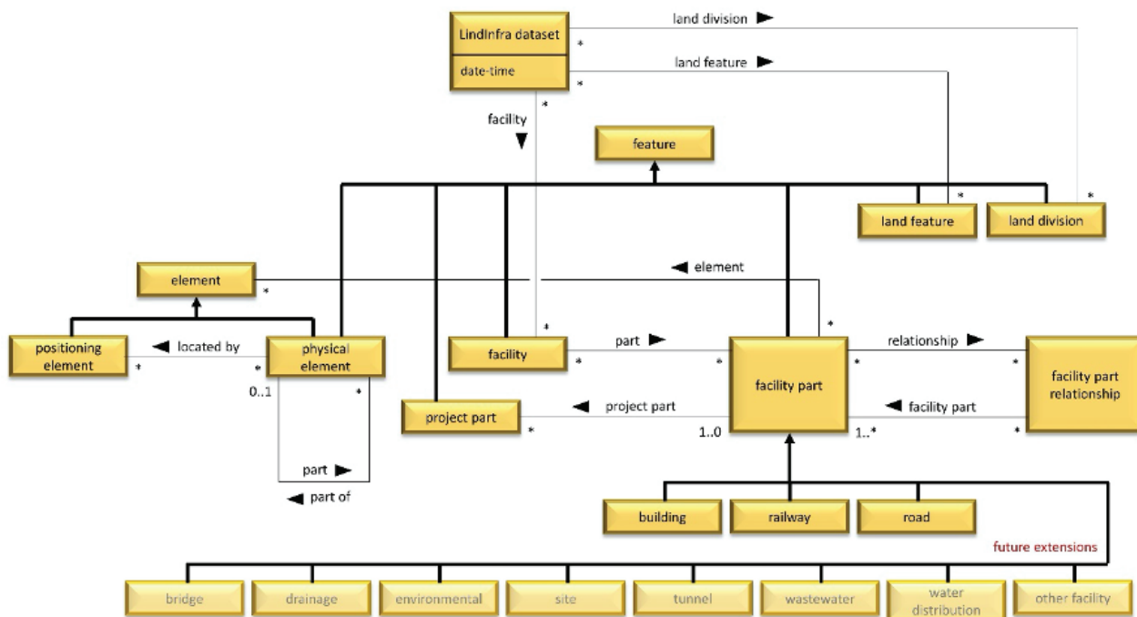
Figure 13 - Top of the LandInfra model
