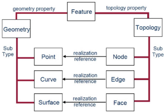
Figure 6 - Geometry and topology in GML
