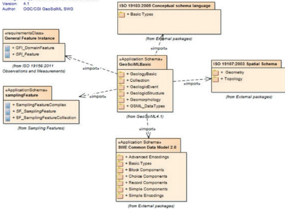
GeoSciMLBasic package dependencies : Package diagram
